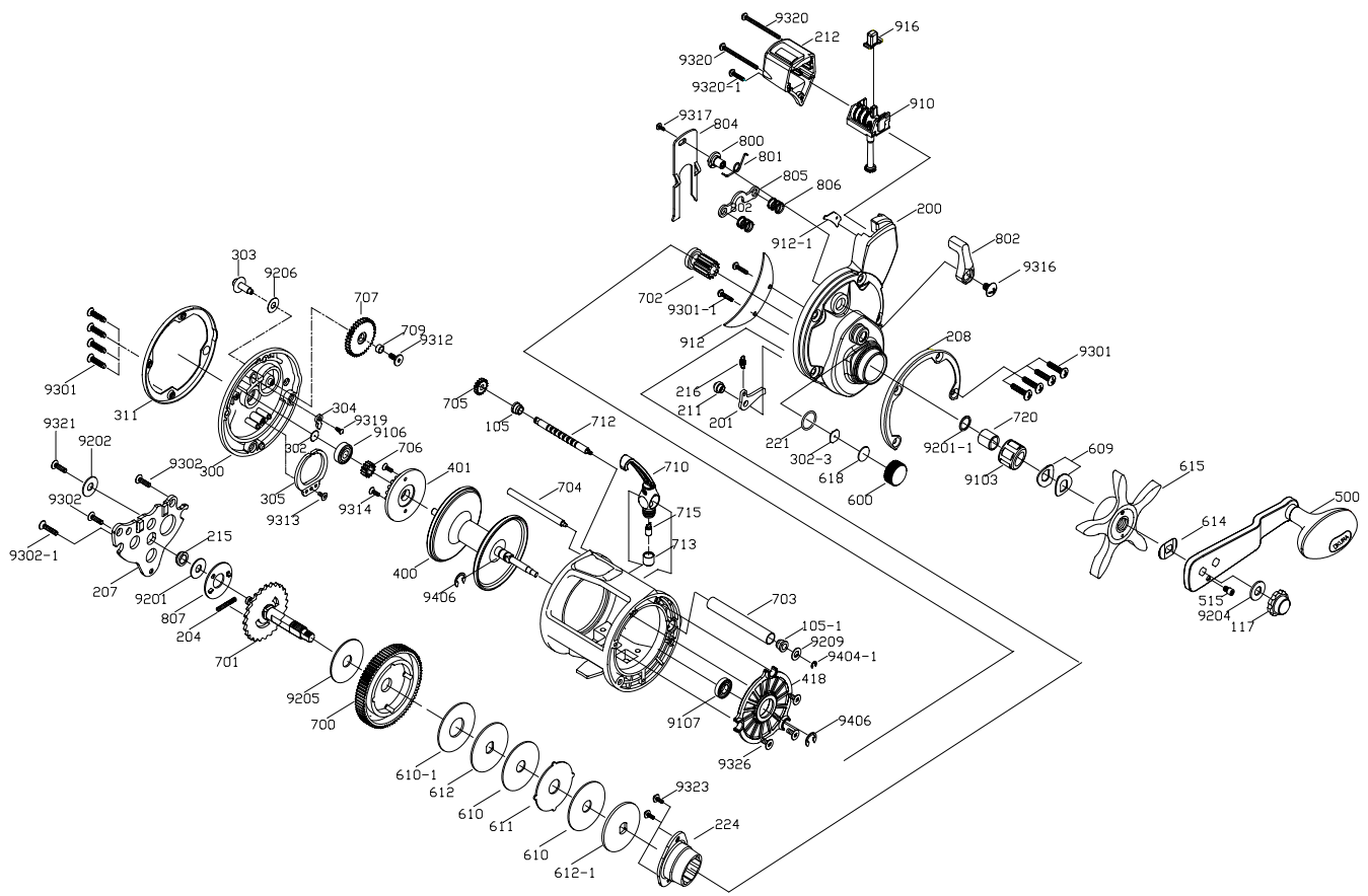
CV - 20D (1 of 2) Spare Parts
